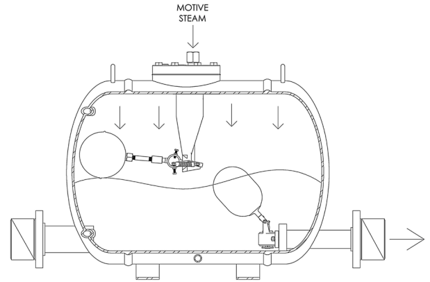
Figure 4: As the body pressurizes the inlet check valve closes. The condensate generated during this time will need to be stored in a receiver or pipe reservoir to prevent water from flooding the heat exchange equipment. When the body pressure is greater than the back pressure, the condensate will be pushed through the trap mechanism and external discharge check valve into the return line.
